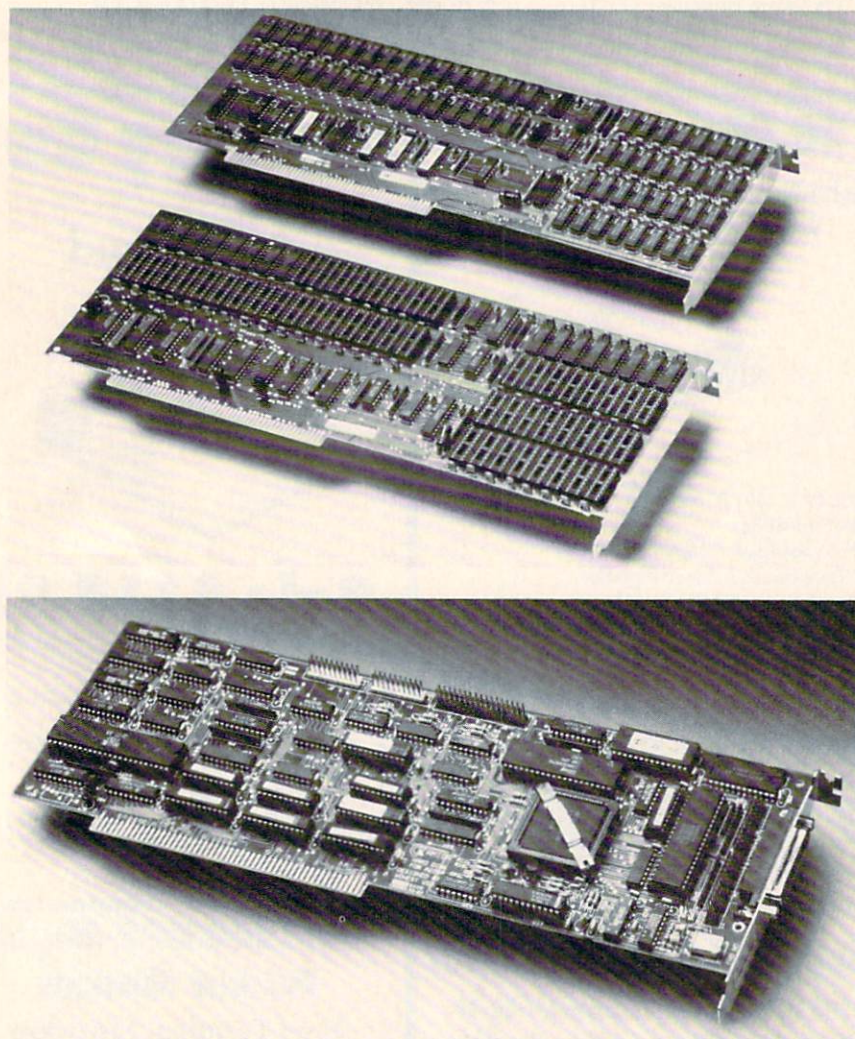
Top: A2058 RAM expansion card configured with 2 (foreground) and 8 megabytes. Bottom: A2090A hard disk controller contains ST-506 and SCSI interfaces.
